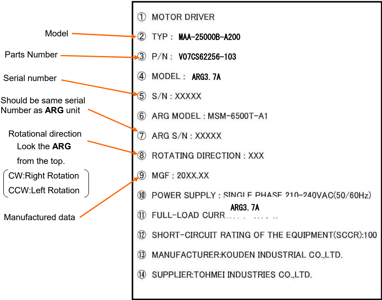
Figure 2-9 Nameplate for the Motor Driver
