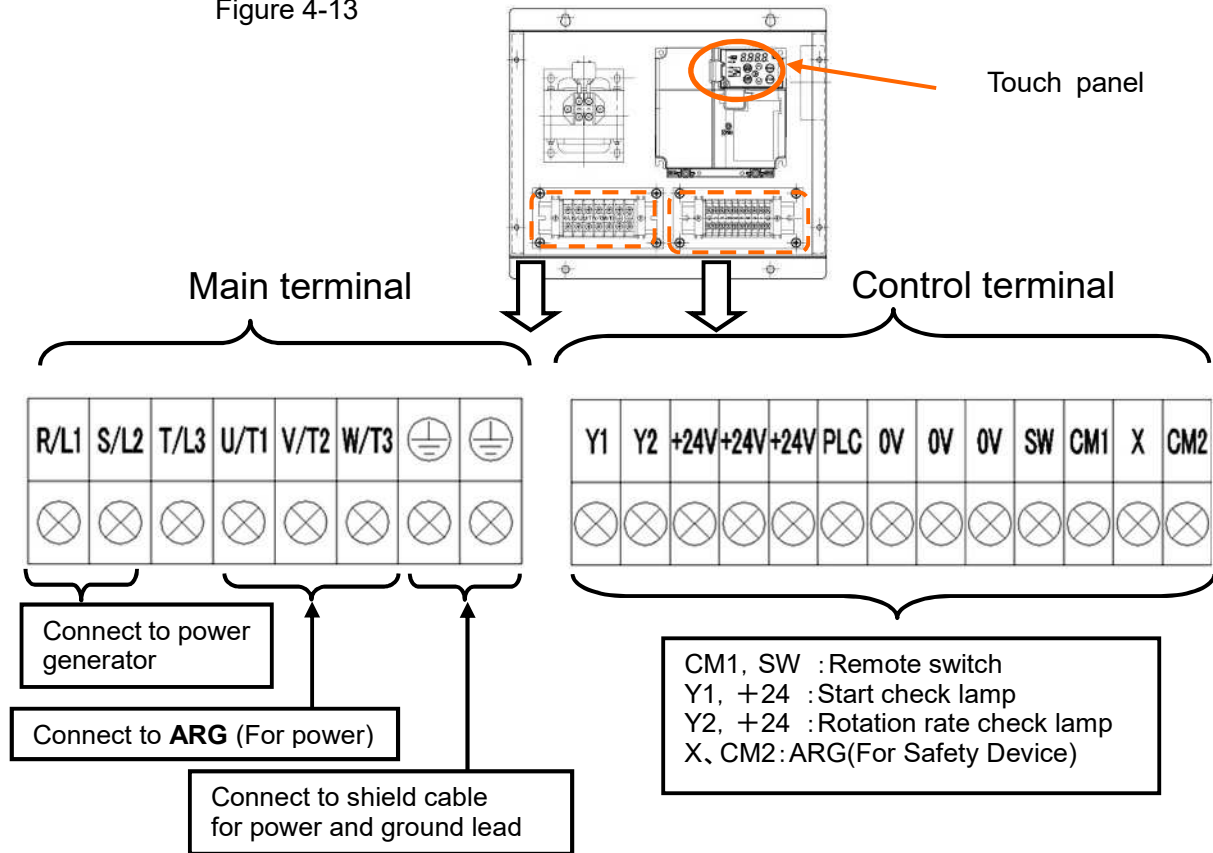
Figure 4-13 Terminal arrangement of the Motor Driver
