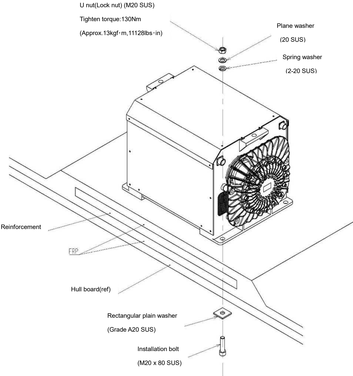
Figure 4 - 2 Installation of the ARG unit
