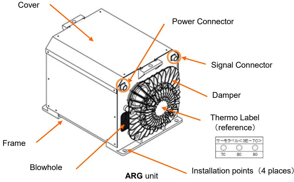
Figure 2-4 ARG unit external view
