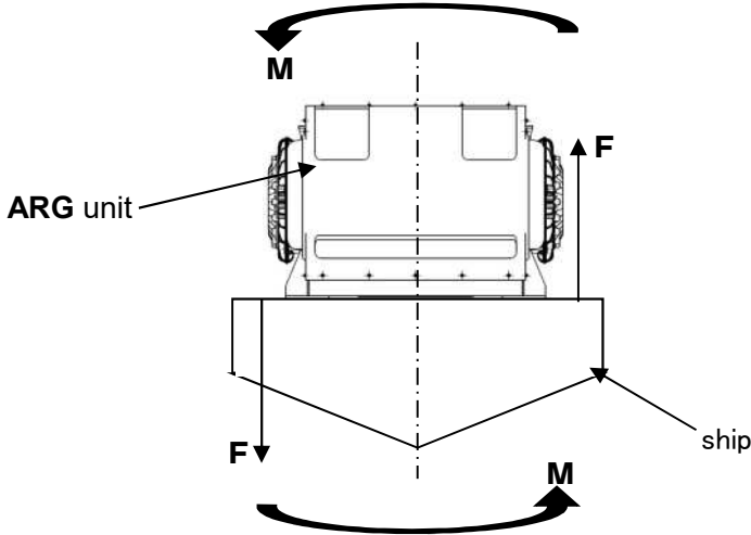
Figure 3-1 Gyro-generated torques (moments)
