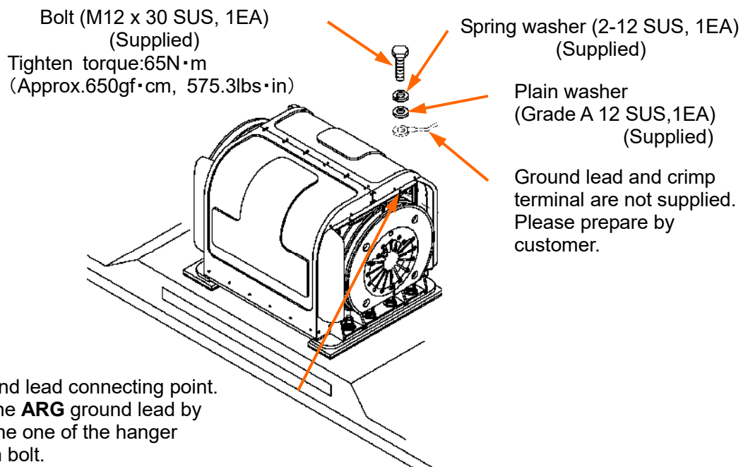
Figure 4-19 Ground lead connection for the ARG unit
