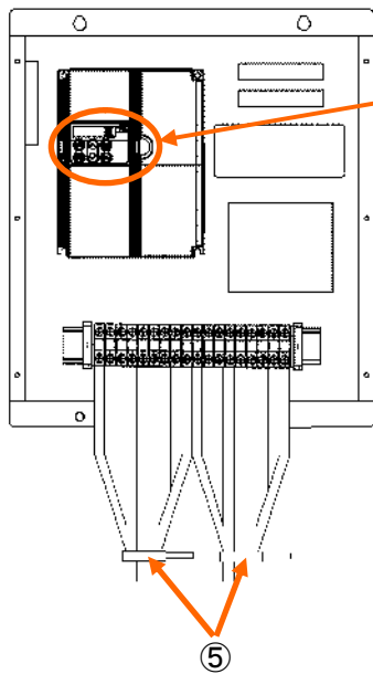
Figure 4-18 How to check the electric voltage just after turned off the Motor Driver
