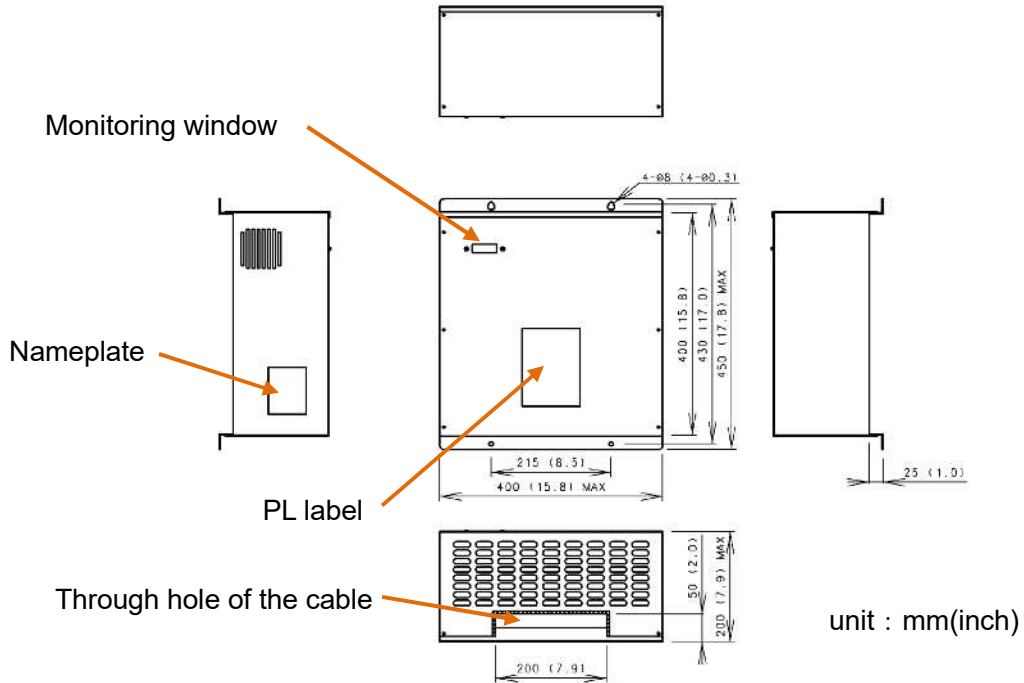
Figure 2-9 Dimensions for Motor Driver
