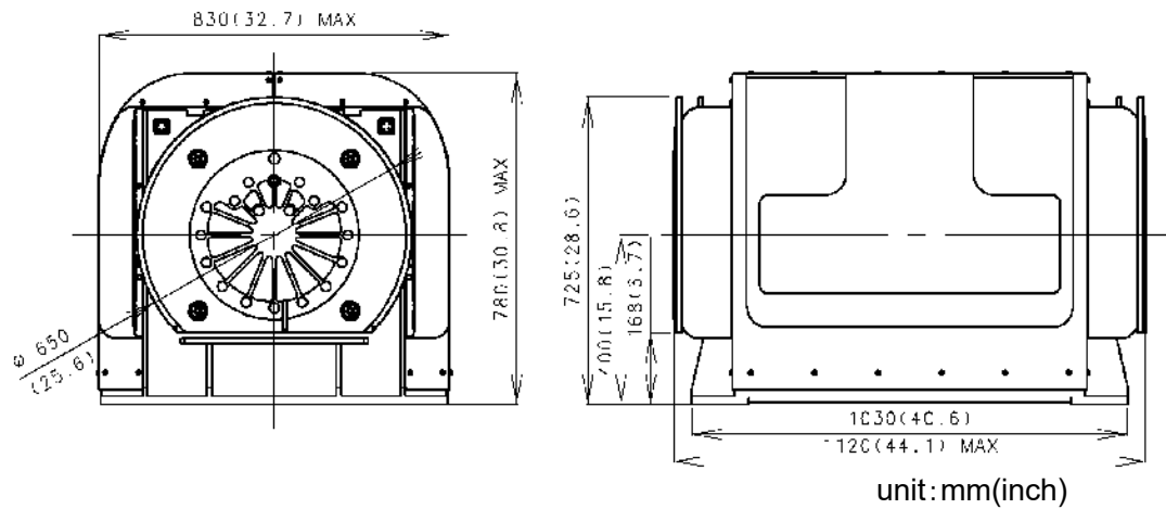
Figure 2-6 Dimensions for the ARG unit
