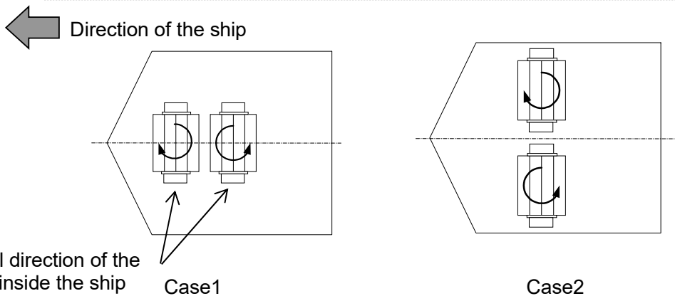
Figure 3-3 Installation direction of the ARG unit
