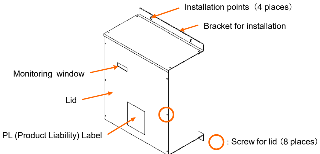
Figure 2-8 Motor Driver External view
