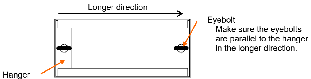
Figure 4-4 Installation direction of eyebolts
