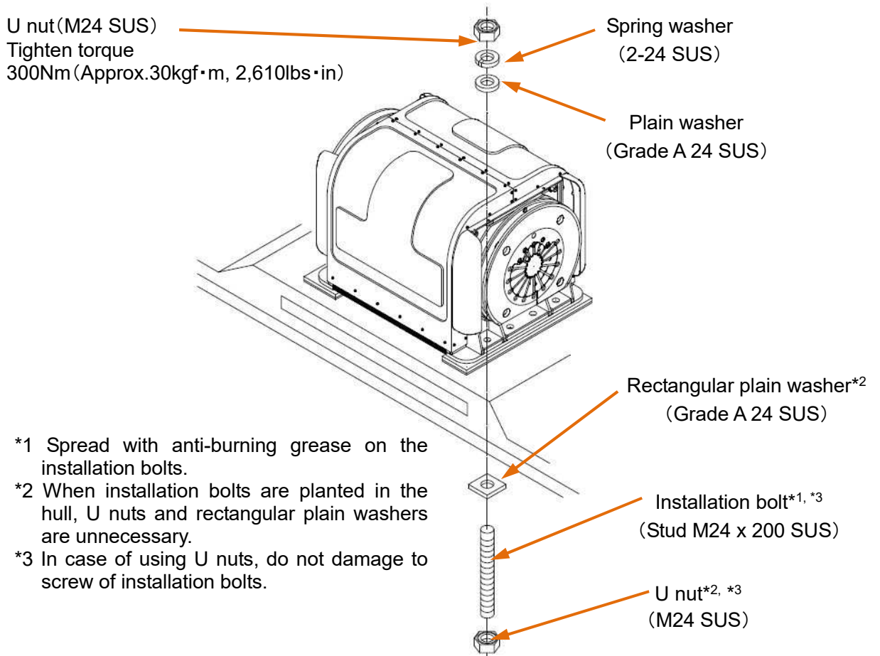
Figure 4-6 Installation of the ARG unit
