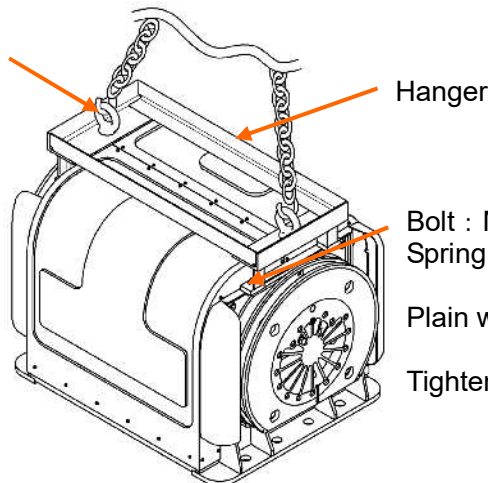
Figure 4-3 Sling up the ARG unit
