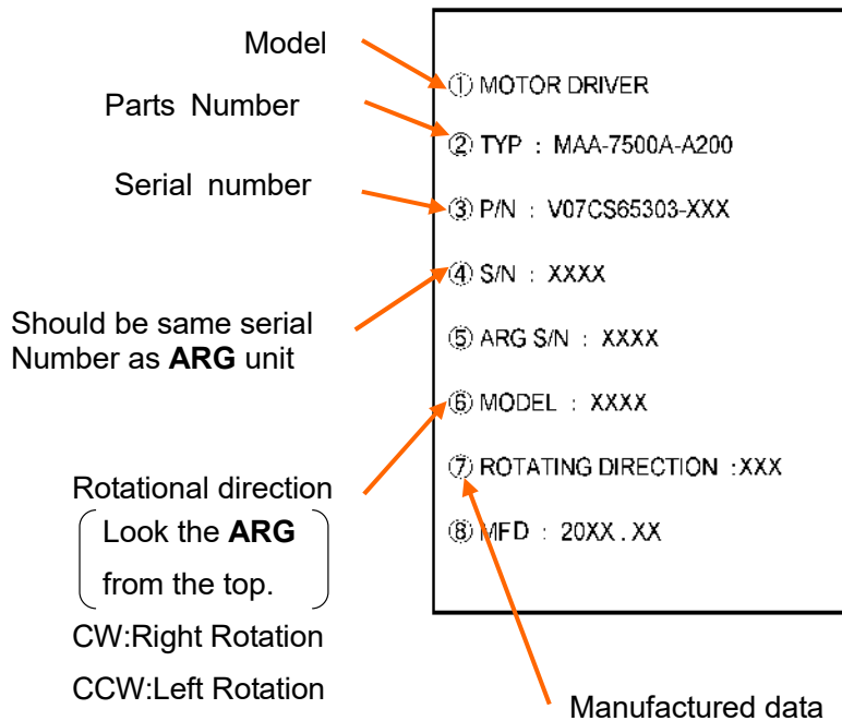
Figure 2-10 Nameplate for the Motor Driver
