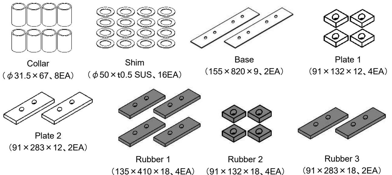
Figure 2-2 Checking of the delivered ARG (No.2)
